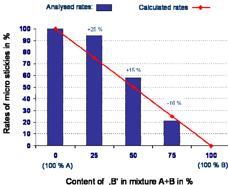
Fig.1 Comparison of analysed and calculated rates of microstickies
